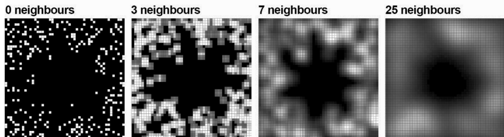
Fig. 6 The effect of spatial summation.
